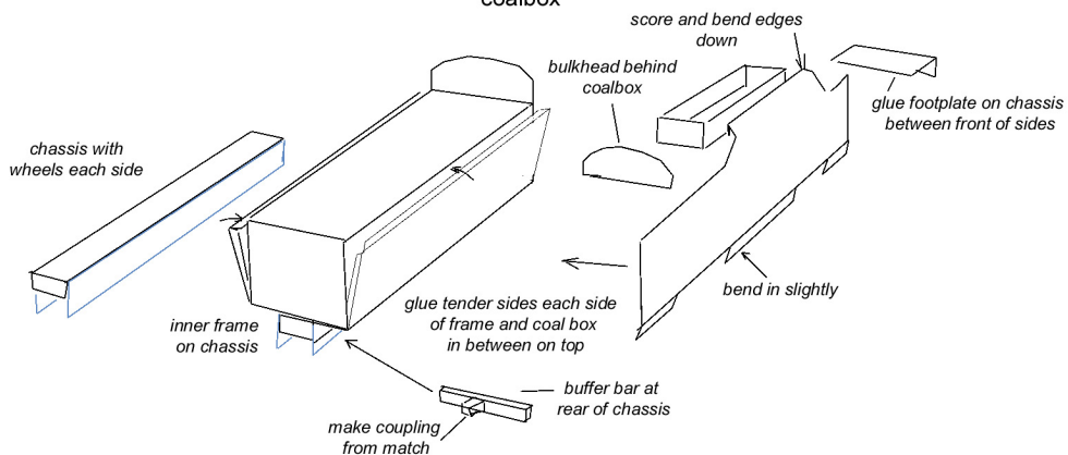
coalbox
